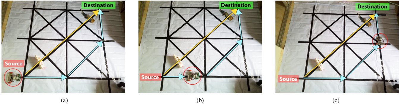
Fig. 5. An illustrative example of testbed simulation (The yellow line denotes the shortest path which is not usable due to the presence of obstacles. The blue lines denote the path followed by the SR): (a) The SR gets the obstacle free shortest path calculated by the FS (b) The SR reaches the next node following the obstacle free path (c) As the environment is unchanged, the previous path is followed
