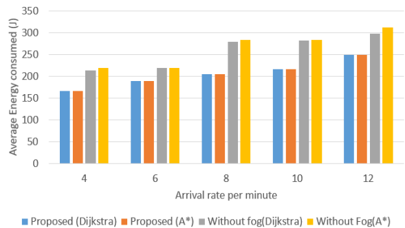
Fig. 8. Energy usage for serving requests
